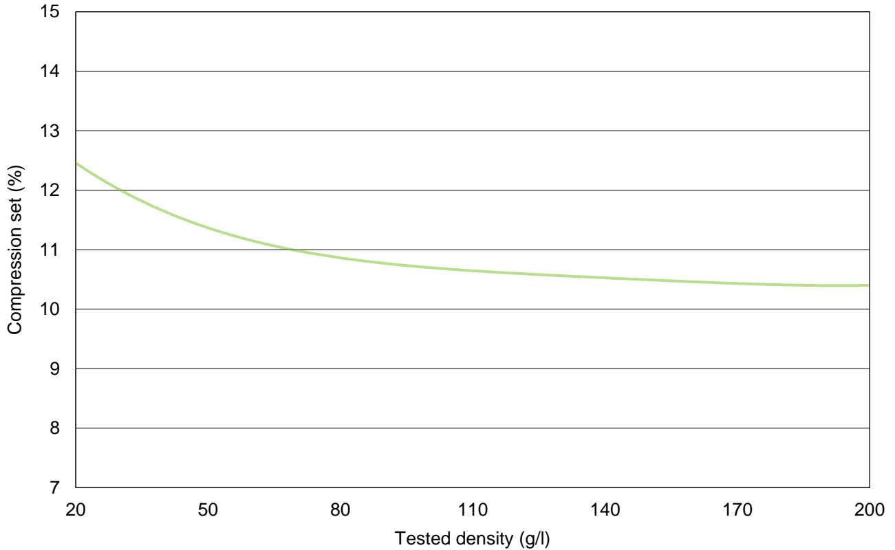
Compression set - ISO 1856 C
